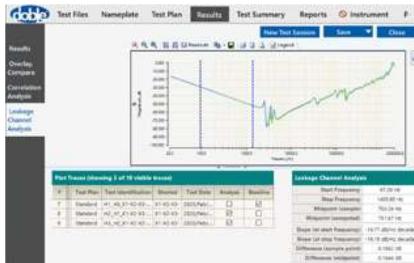
Results of automated Leakage Channel Analysis presented to the user.
